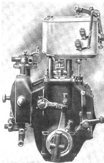
Rear View of 1910 White Engine
